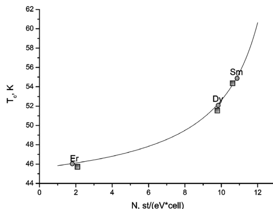
Figure 4. Dependence of T_c on the density of states on the Fermi surface N(E_f) for ReFeAsO [13] (○—theory, □—experiment).
