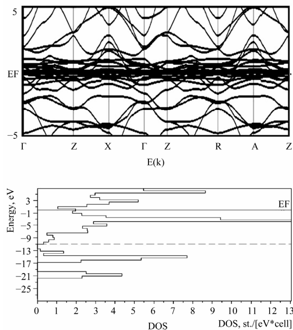
Figure 3. Results of our calculations of the band structure and the density of states for ErFeAsO with T_c = 46 K.
