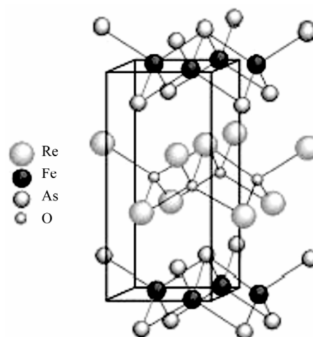
Figure 1. Crystalline structure of ReFeAsO.
