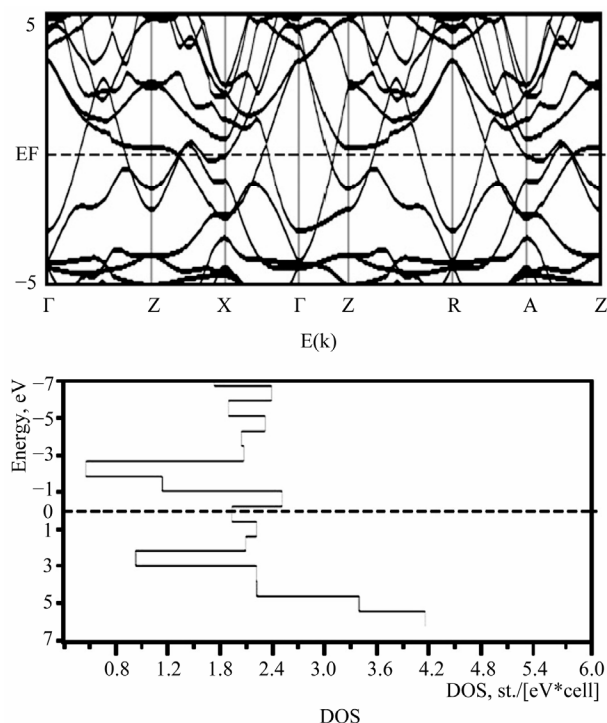
Figure 2. Results of our calculations of the band structure and the density of states for SmFeAsO with T_c = 55.0 K.
